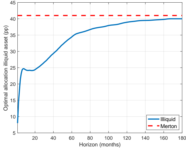
Figure 4. No-trading region
